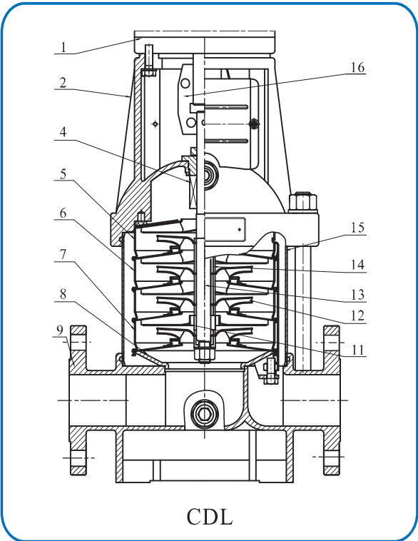
截面图 CDL,CDLF8,10,12,15,16,20
